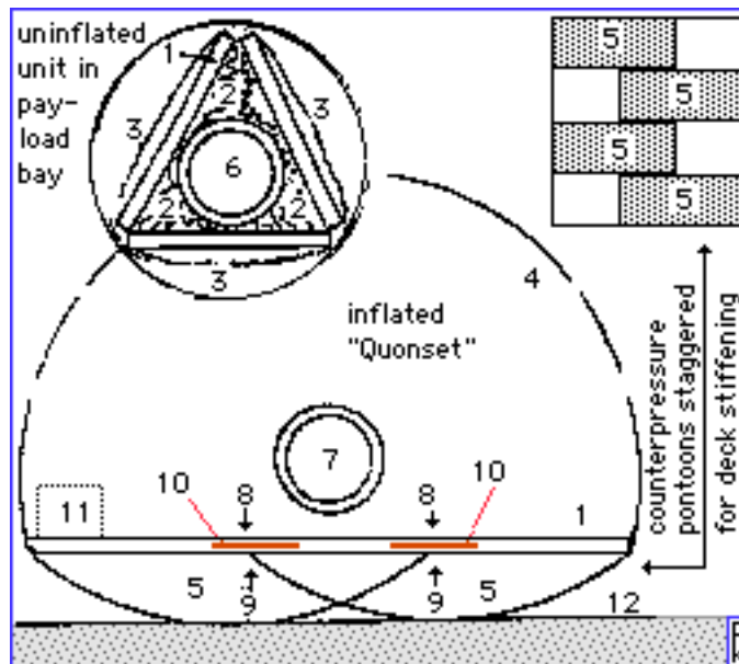
Figure 6. QUONSET: [1] Hinged 3-section floor deck. [2] uninflated quonset roof/wall [3] uninflated floor support pontoons [4] inflated quonset roof/wall [5] Inflated floor support pontoons [6] In transit position of docking module [7] Docking tunnel in end wall [8] Downward air pressure on hinges [9] Counterbalance pressure on hinges [10] Contingency stiffening bars [11] Representative pull-up feature [12] Ground contour before shielding
