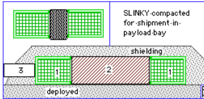
Figure 5: The Slinky: [1] Pair of rigid end caps, outfitted with build-in features and equipment. [2] expandable slinky module (unfurnished). [3] docking tunnel.
